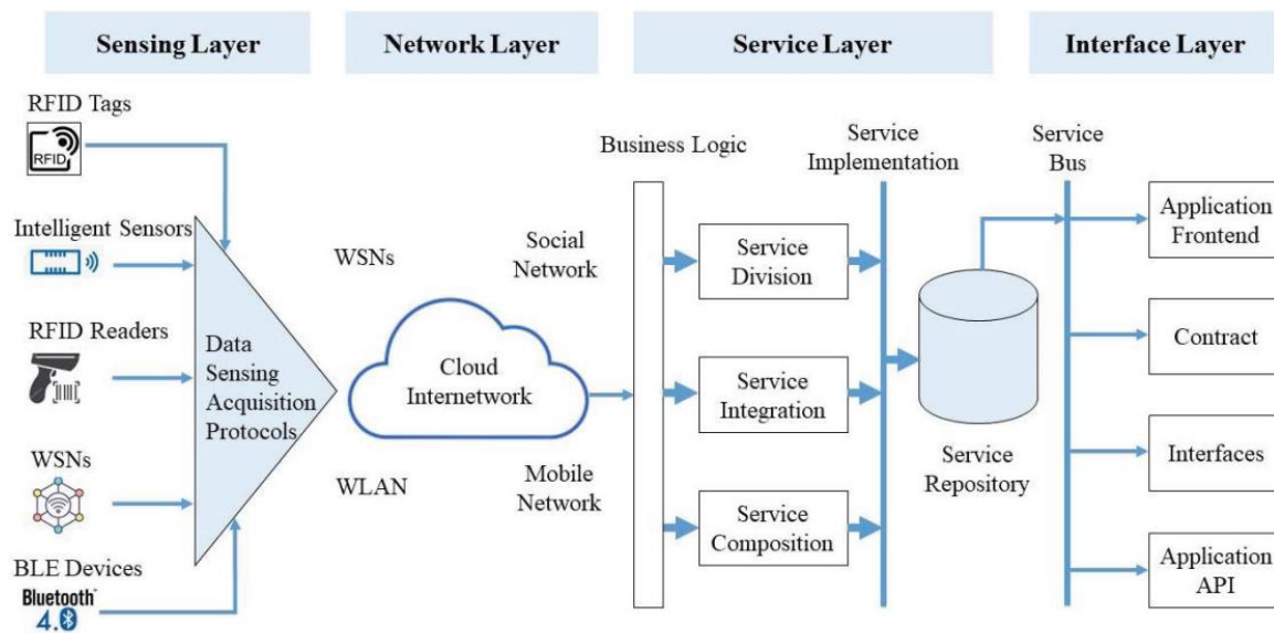
Fig.11.7: Architectural Layers of Internet of Things
