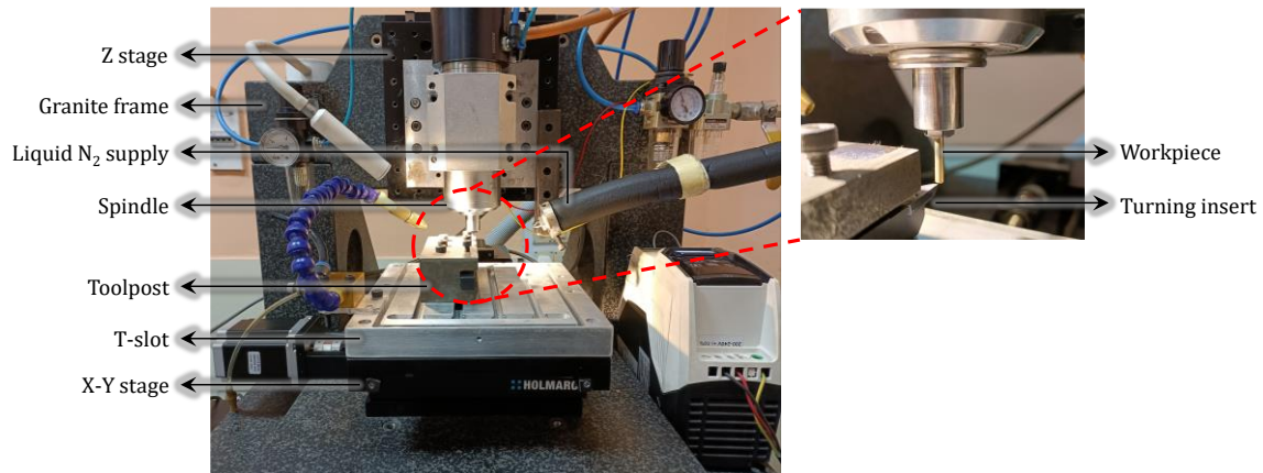
Fig. 1 The experimental setup (Micromachining center model "V60")
