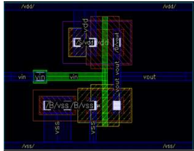
Fig. 5 Layout Design in GPDK45
